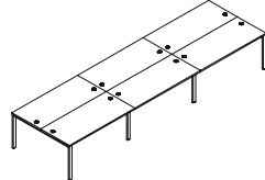
BG064 / VBG064 4800/1400/758
